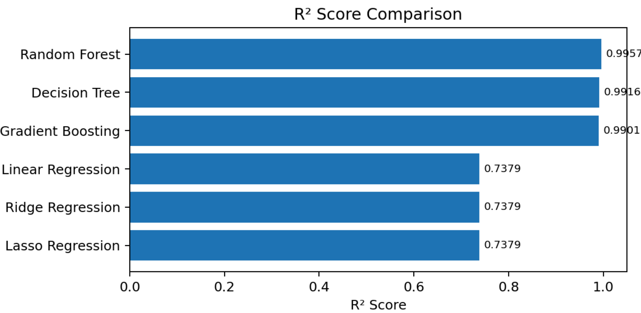
Figure 4.2 — R² Score Comparison of Regression Models
