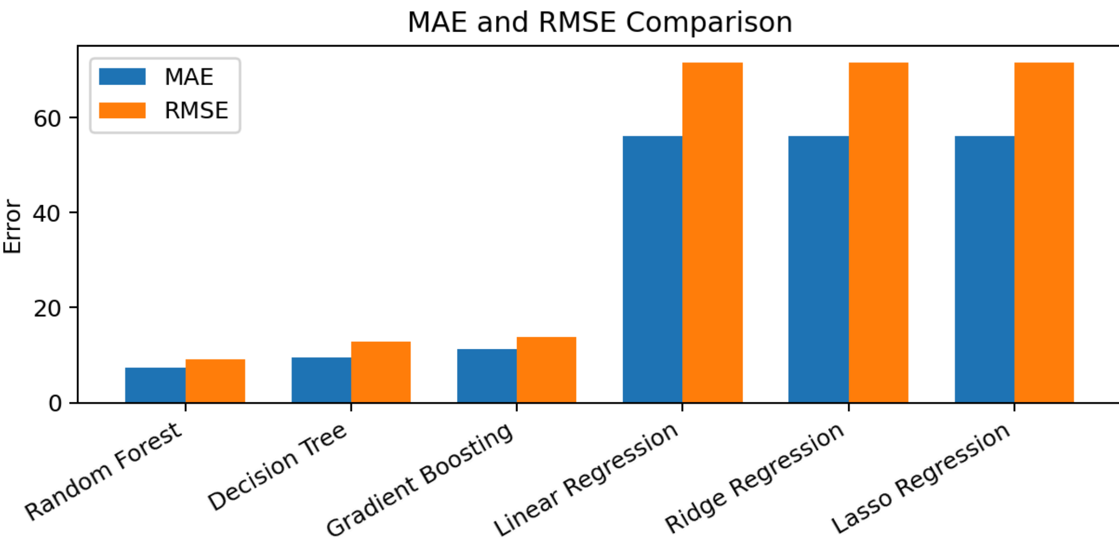
Figure 4.3 — Error Comparison of Regression Models
